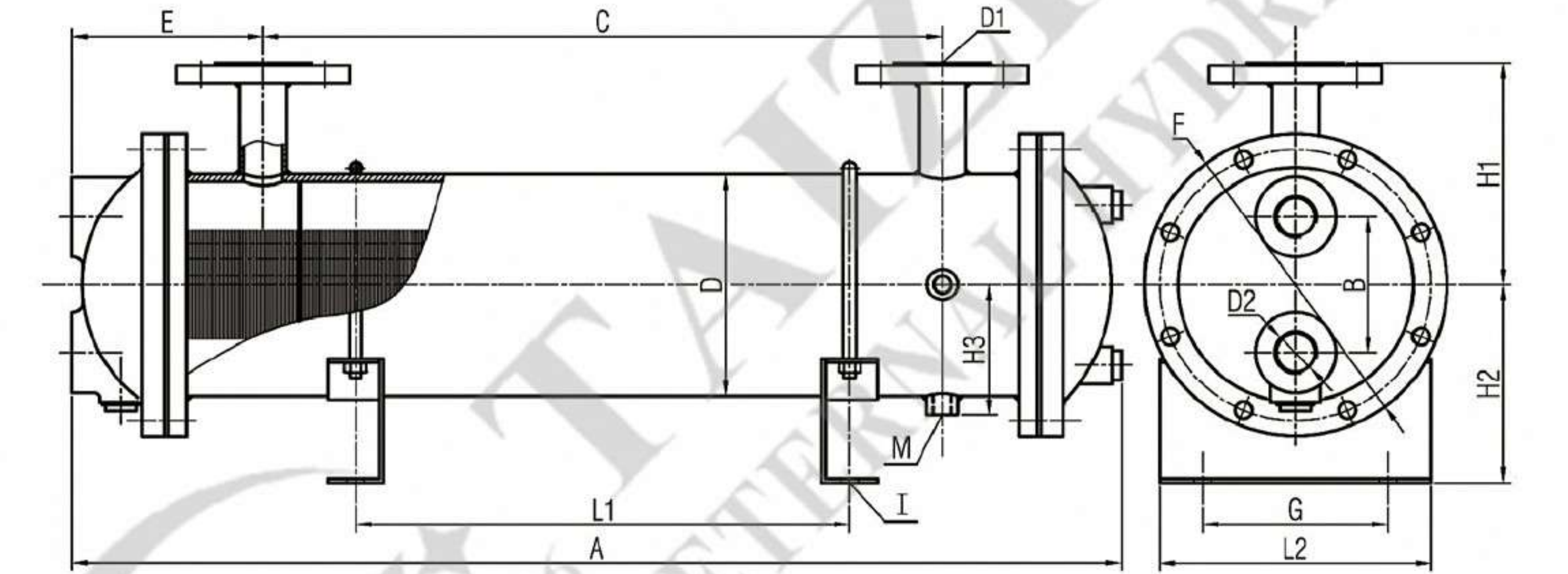
GLP系列水冷却器结构图 GLP Water Cooler Specifications And Dimensions
