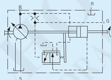
带机械行程限位的恒功率变量LV……M Constant power control with mechanical stroke limiter
