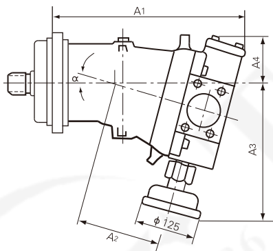
手轮朝下 handwheel downwards
