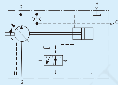
恒功率变量LV Constant power control
