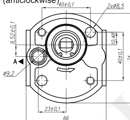
Rotation "C" - (clockwise)
